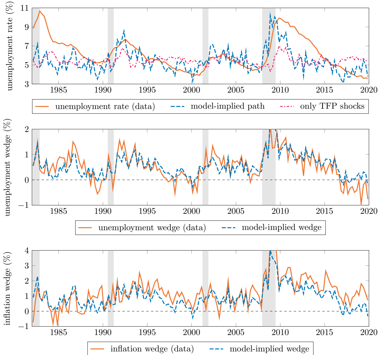
Figure 6: Data and model-implied time series for unemployment and belief wedges.
